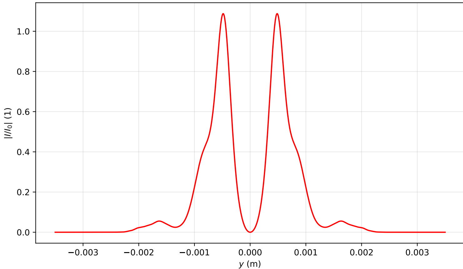
Intensity profile I(x=0, y, z=1.672)/I_0 , \text{Pin}=7.0\text{Pcr} , artificial time
